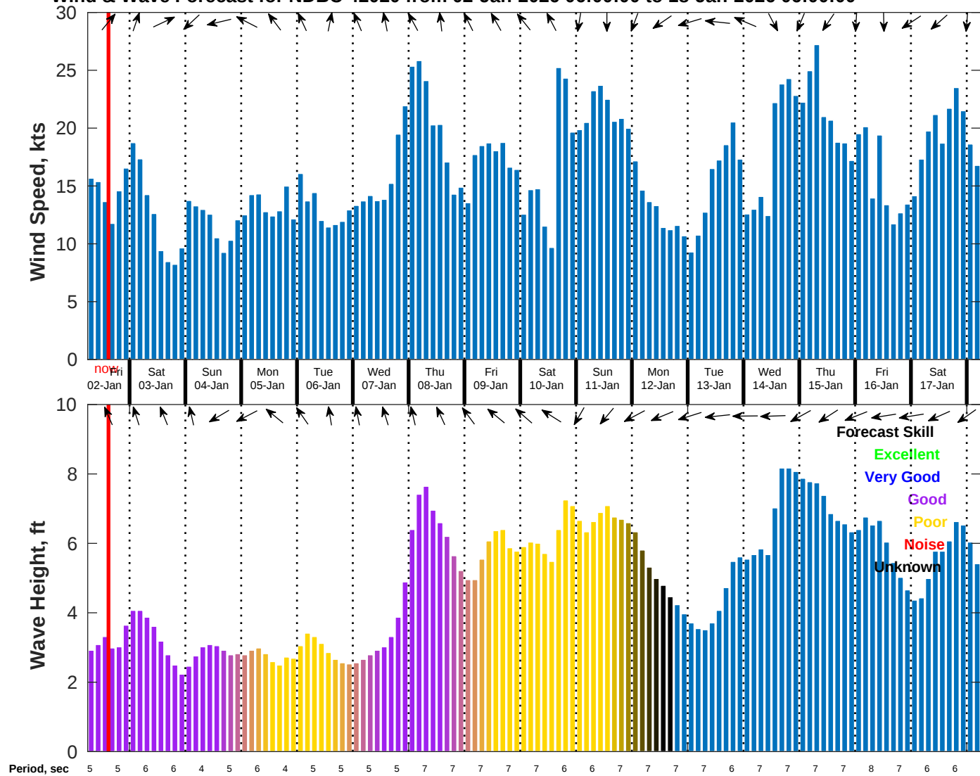
Wind & Wave Forecast for NDBC 42020 from 02-Jan-2026 06:00:00 to 18-Jan-2026 06:00:00
