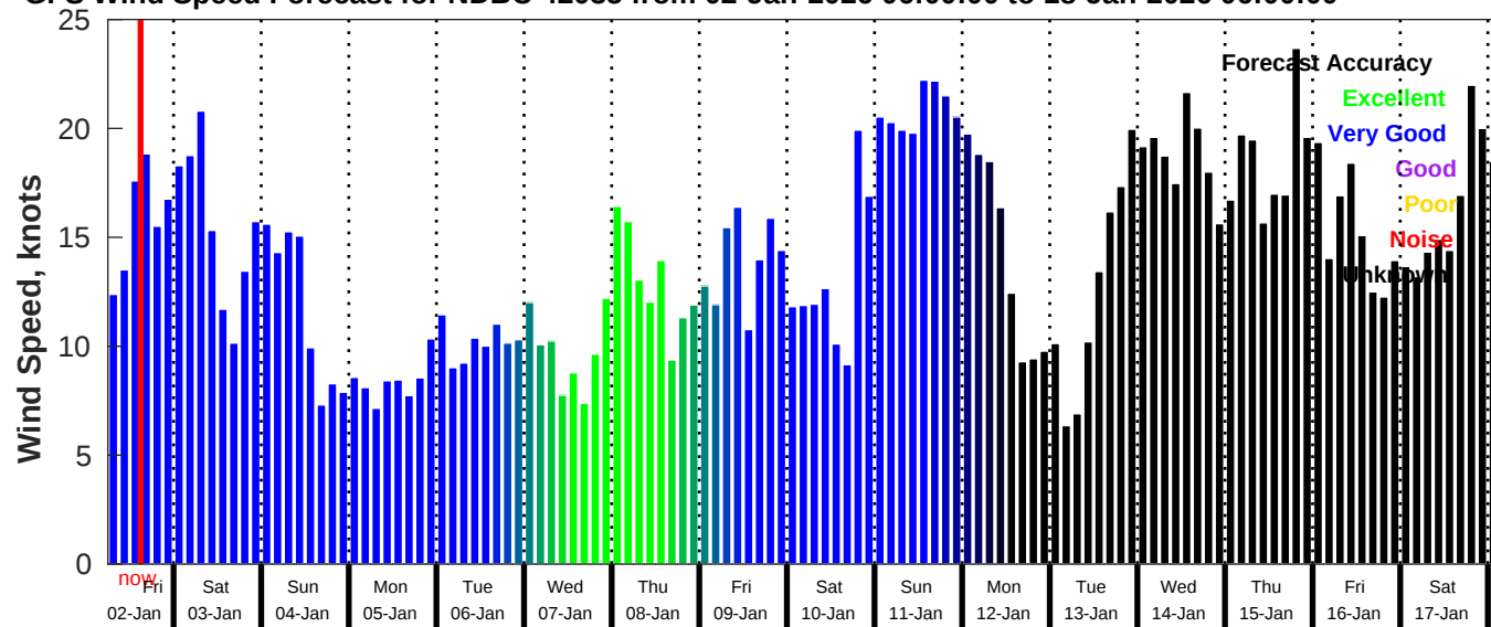
GFS Wind Speed Forecast for NDBC 42035 from 02-Jan-2026 06:00:00 to 18-Jan-2026 06:00:00
