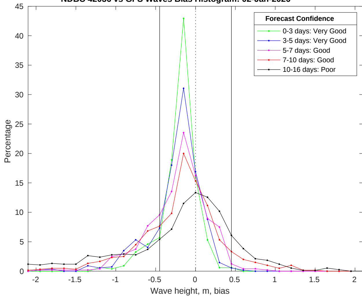
NDBC 42036 vs GFS Waves Bias Histogram: 02-Jan-2026
