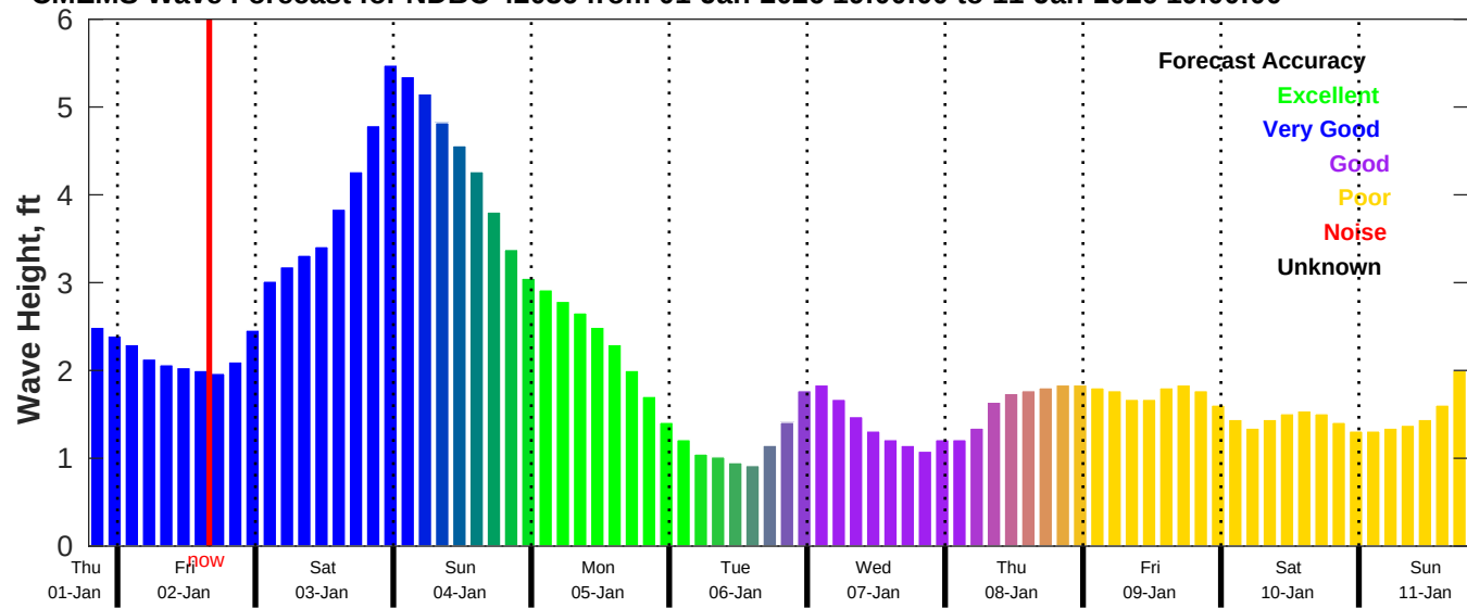
CMEMS Wave Forecast for NDBC 42036 from 01-Jan-2026 19:00:00 to 11-Jan-2026 19:00:00
