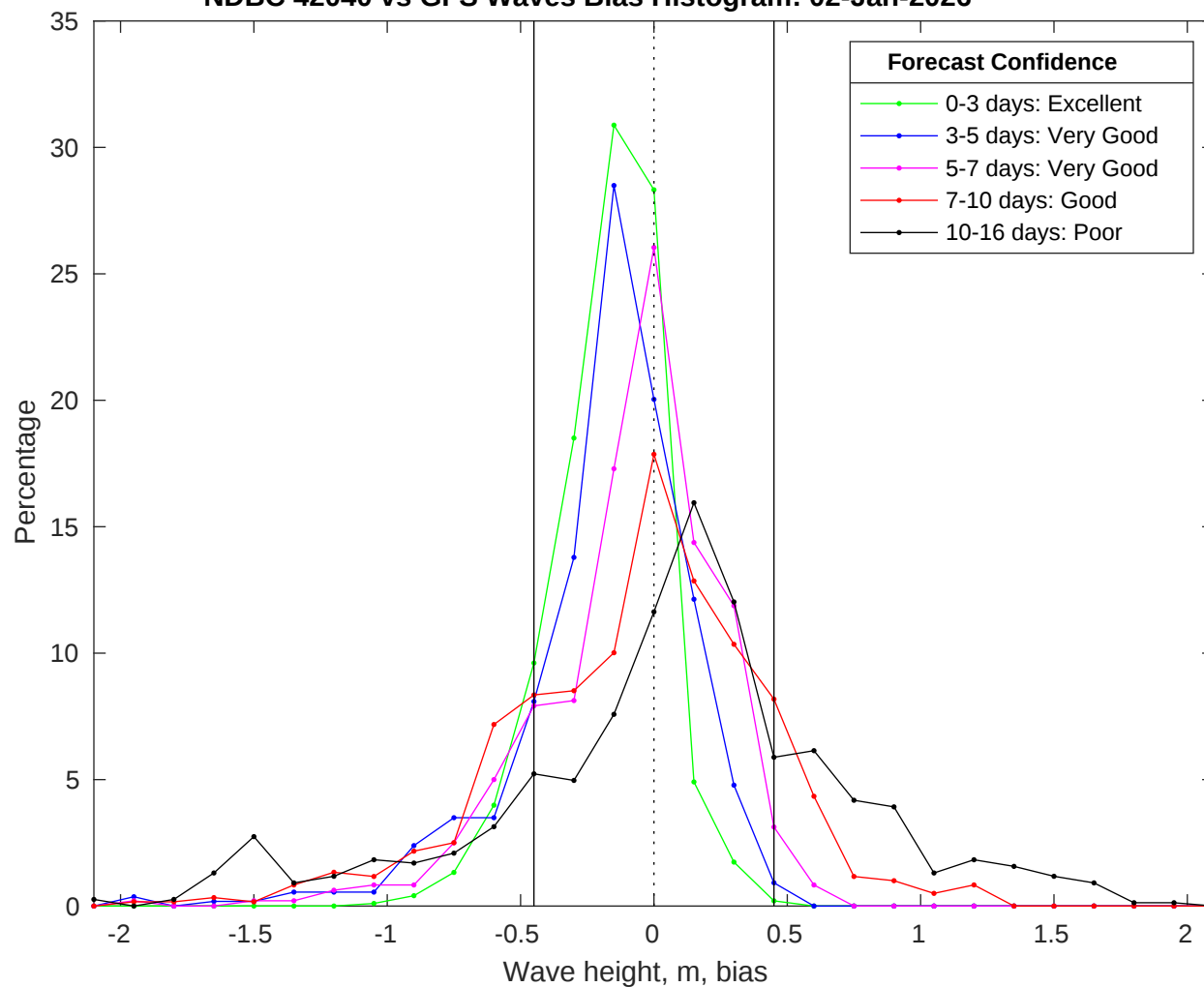
NDBC 42040 vs GFS Waves Bias Histogram: 02-Jan-2026
