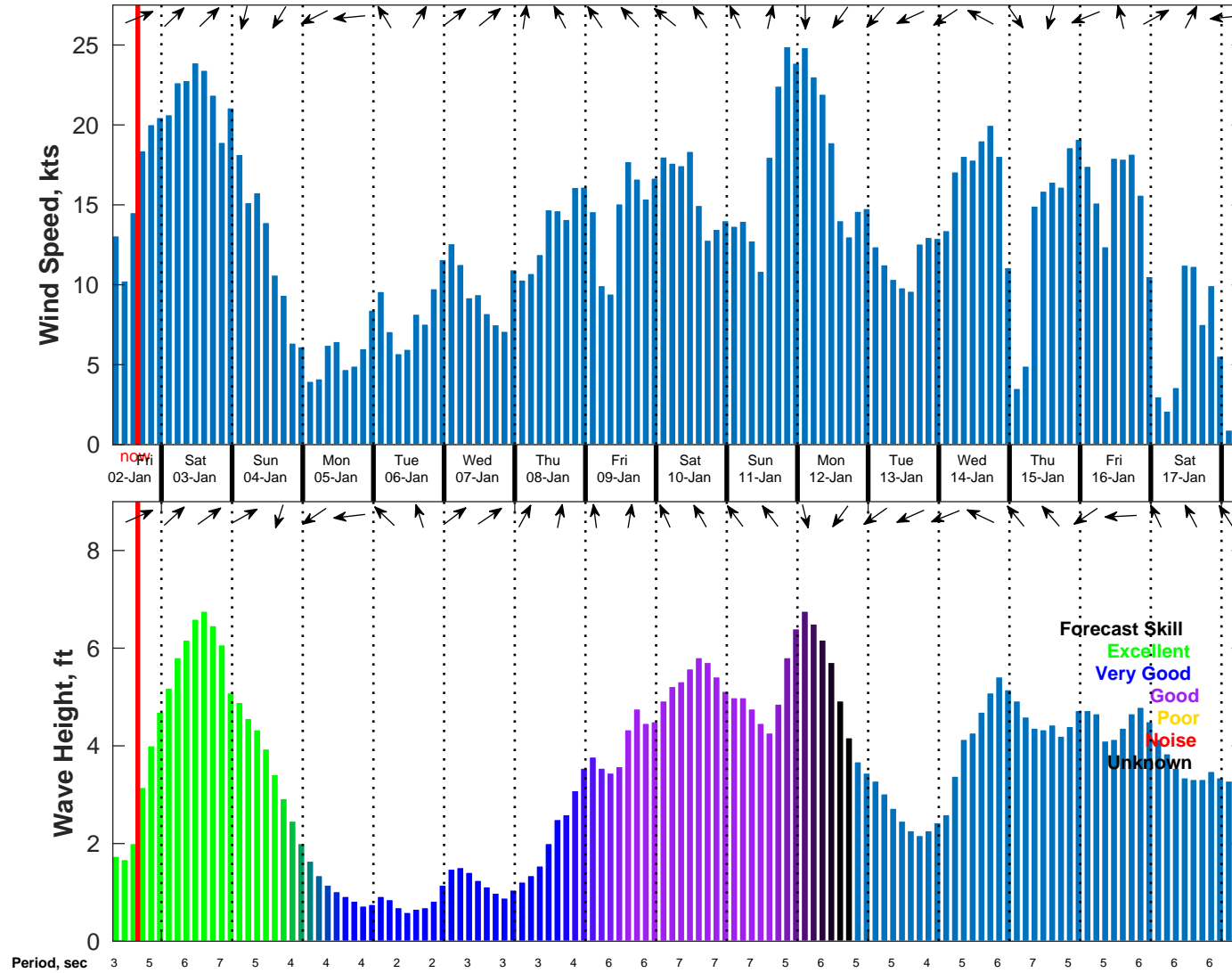
Wind & Wave Forecast for NDBC 42040 from 02-Jan-2026 07:00:00 to 18-Jan-2026 07:00:00
