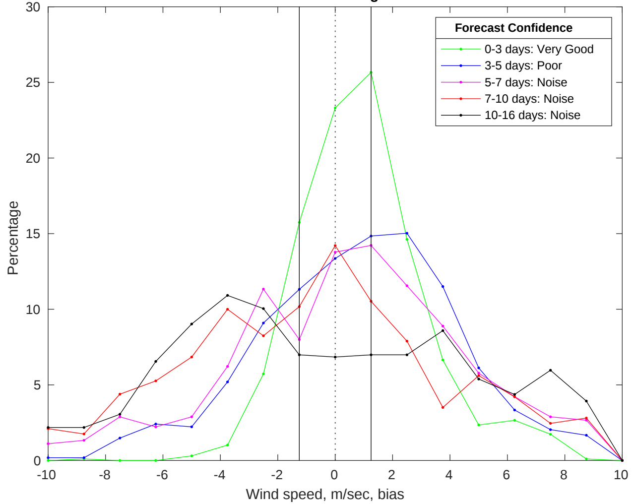
NDBC 44008 vs GFS Winds Bias Histogram: 02-Jan-2026
