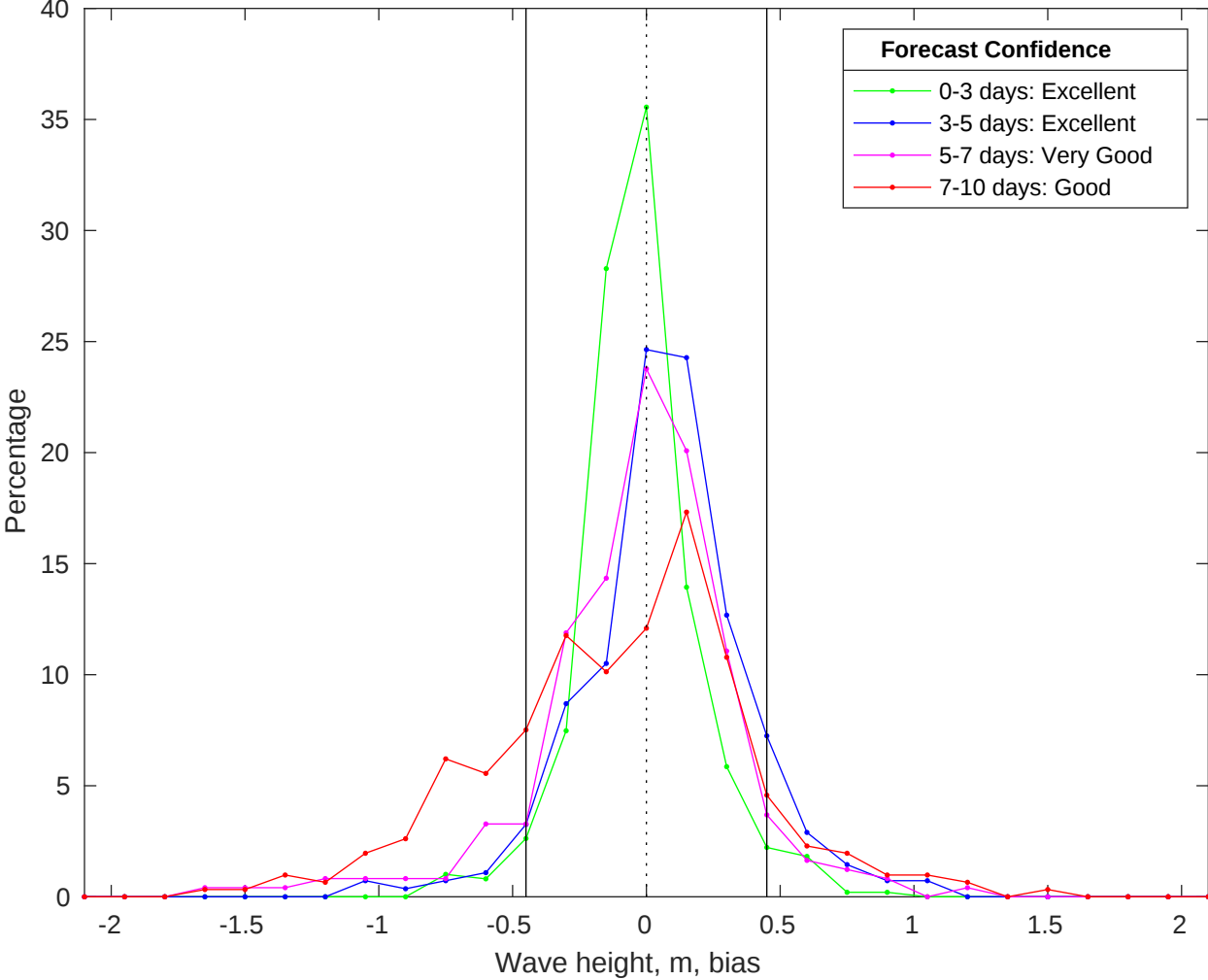
NDBC 46011 vs CMEMS Waves Bias Histogram: 02-Jan-2026
