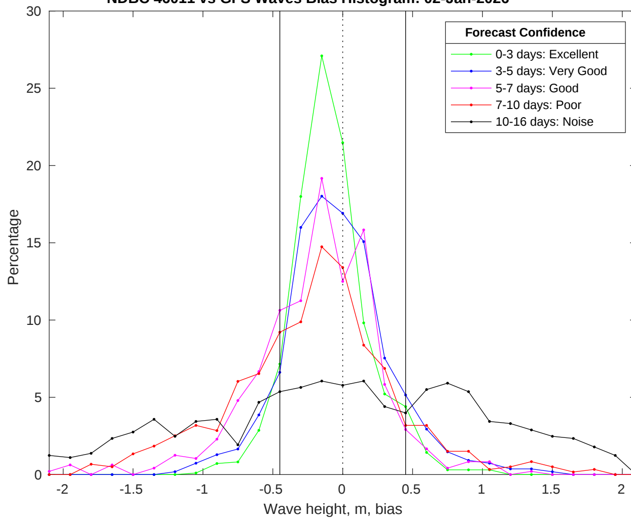
NDBC 46011 vs GFS Waves Bias Histogram: 02-Jan-2026
