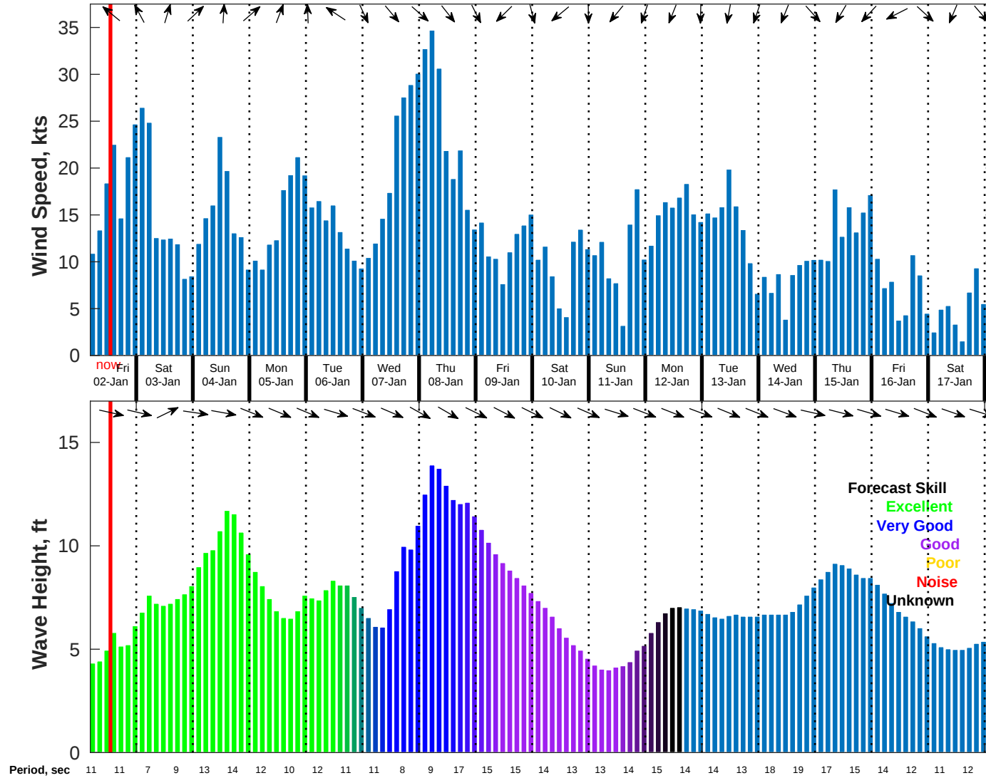
Wind & Wave Forecast for NDBC 46011 from 02-Jan-2026 04:00:00 to 18-Jan-2026 04:00:00
