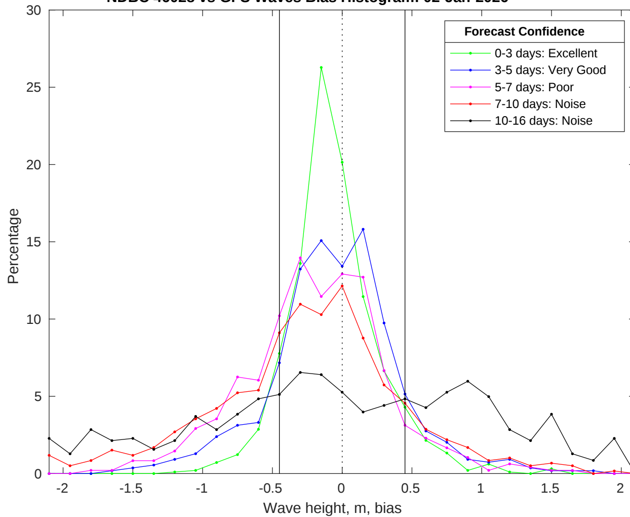
NDBC 46028 vs GFS Waves Bias Histogram: 02-Jan-2026
