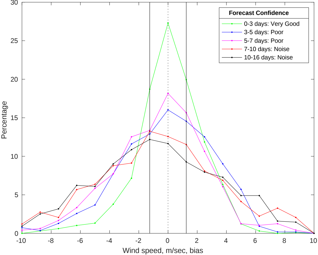
NDBC 46028 vs GFS Winds Bias Histogram: 02-Jan-2026
