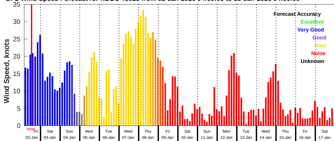
GFS Wind Speed Forecast for NDBC 46028 from 02-Jan-2026 04:00:00 to 18-Jan-2026 04:00:00
