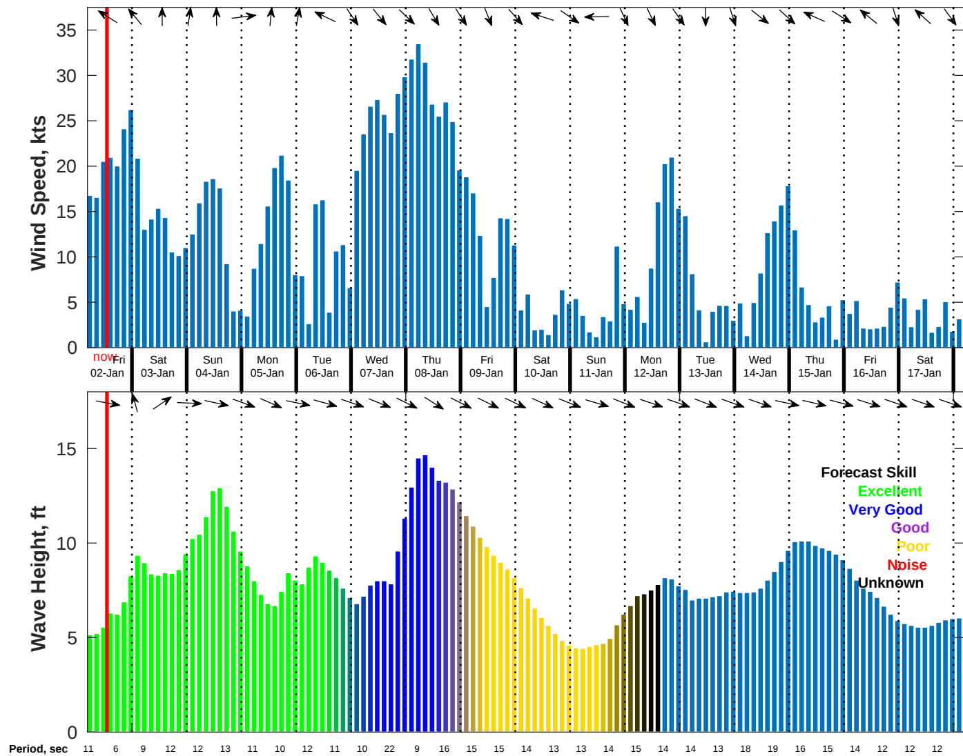
Wind & Wave Forecast for NDBC 46028 from 02-Jan-2026 04:00:00 to 18-Jan-2026 04:00:00
