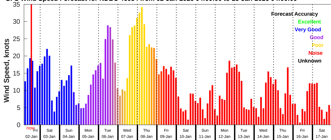
GFS Wind Speed Forecast for NDBC 46054 from 02-Jan-2026 04:00:00 to 18-Jan-2026 04:00:00
