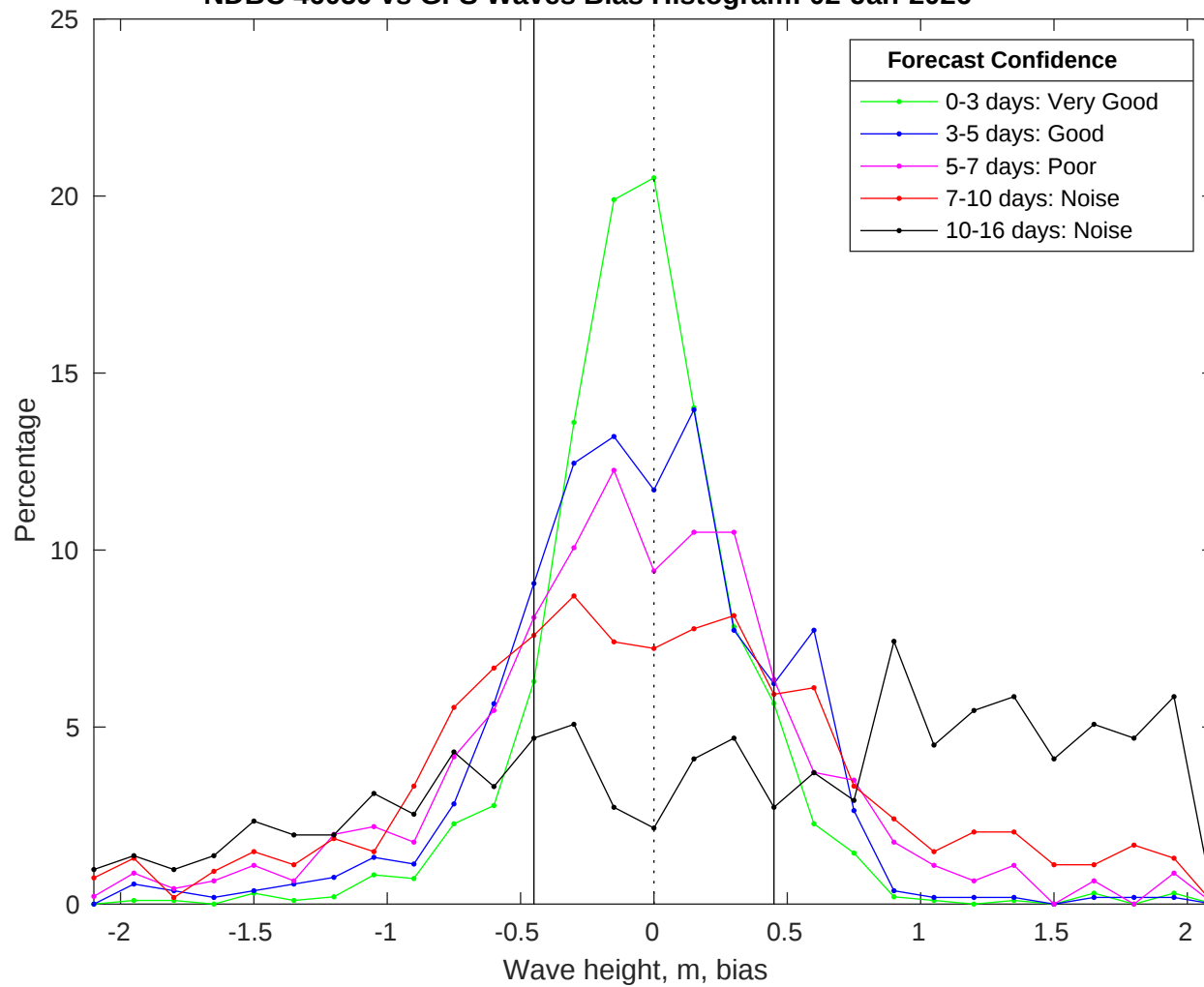
NDBC 46059 vs GFS Waves Bias Histogram: 02-Jan-2026
