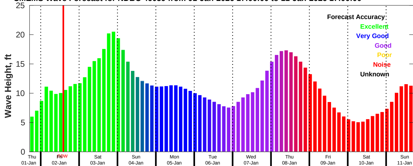
CMEMS Wave Forecast for NDBC 46059 from 01-Jan-2026 17:00:00 to 11-Jan-2026 17:00:00
