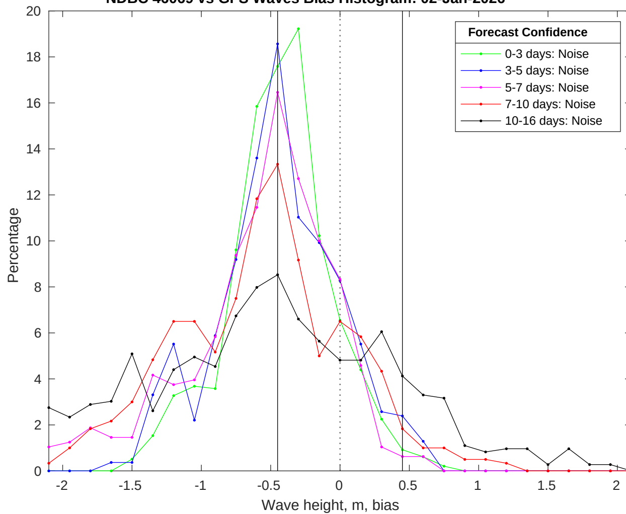
NDBC 46069 vs GFS Waves Bias Histogram: 02-Jan-2026
