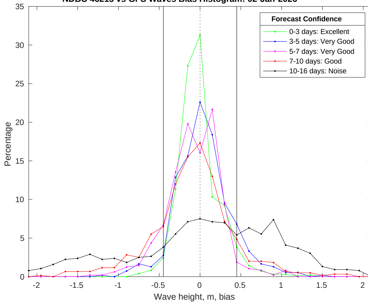
NDBC 46215 vs GFS Waves Bias Histogram: 02-Jan-2026
