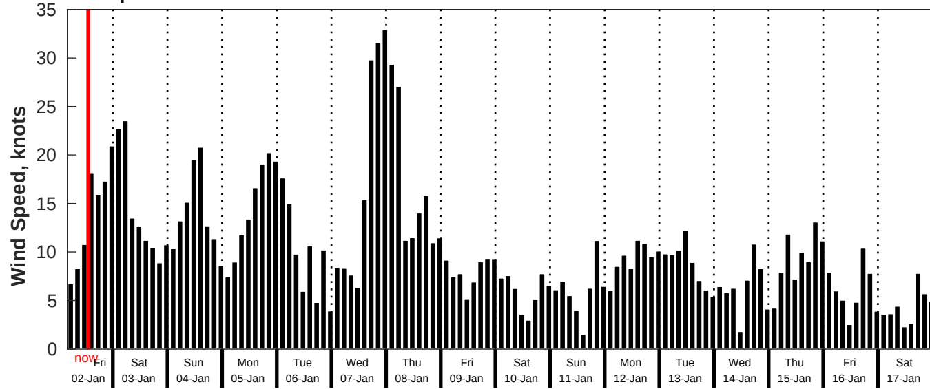
GFS Wind Speed Forecast for NDBC 46215 from 02-Jan-2026 04:00:00 to 18-Jan-2026 04:00:00
