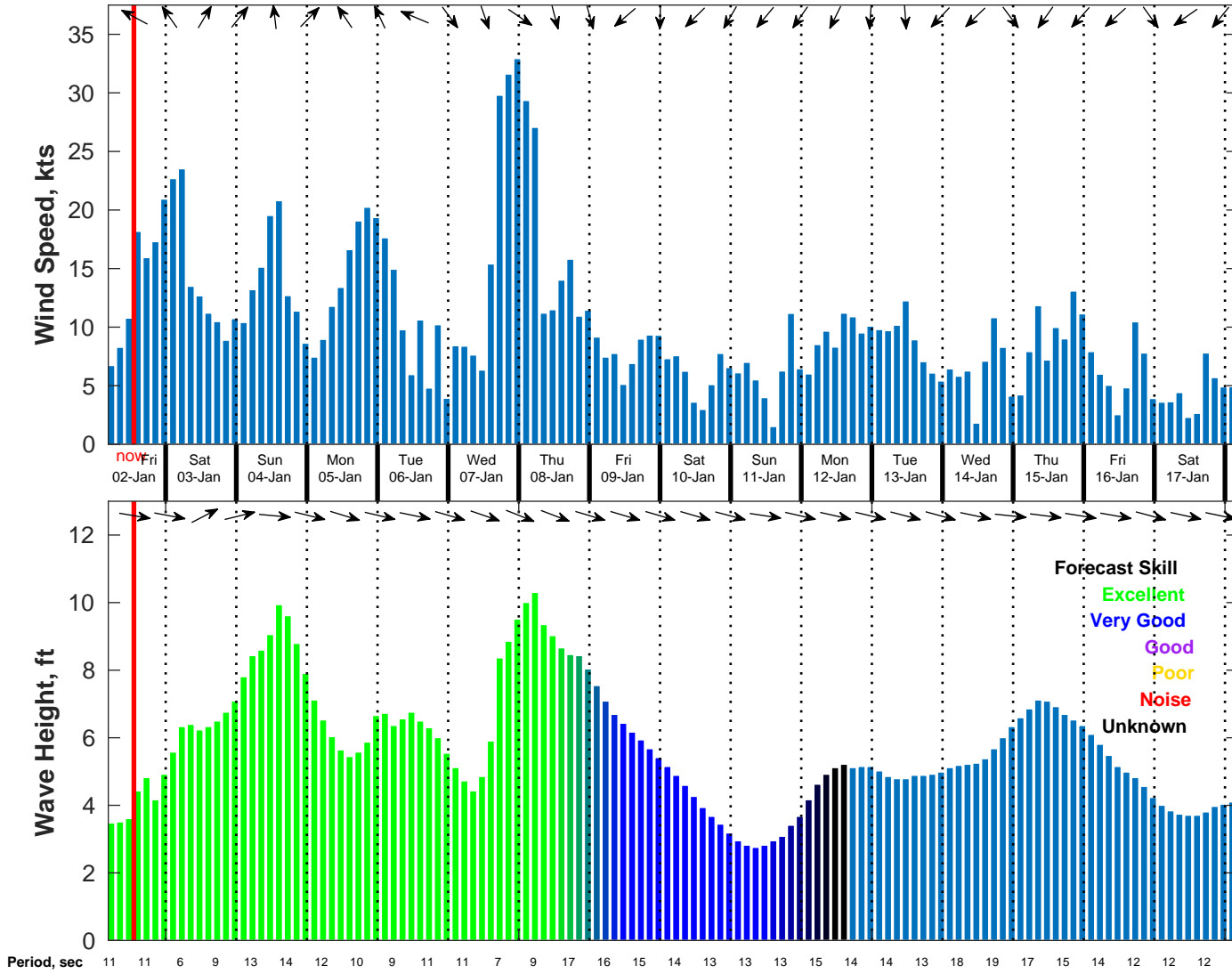
Wind & Wave Forecast for NDBC 46215 from 02-Jan-2026 04:00:00 to 18-Jan-2026 04:00:00
