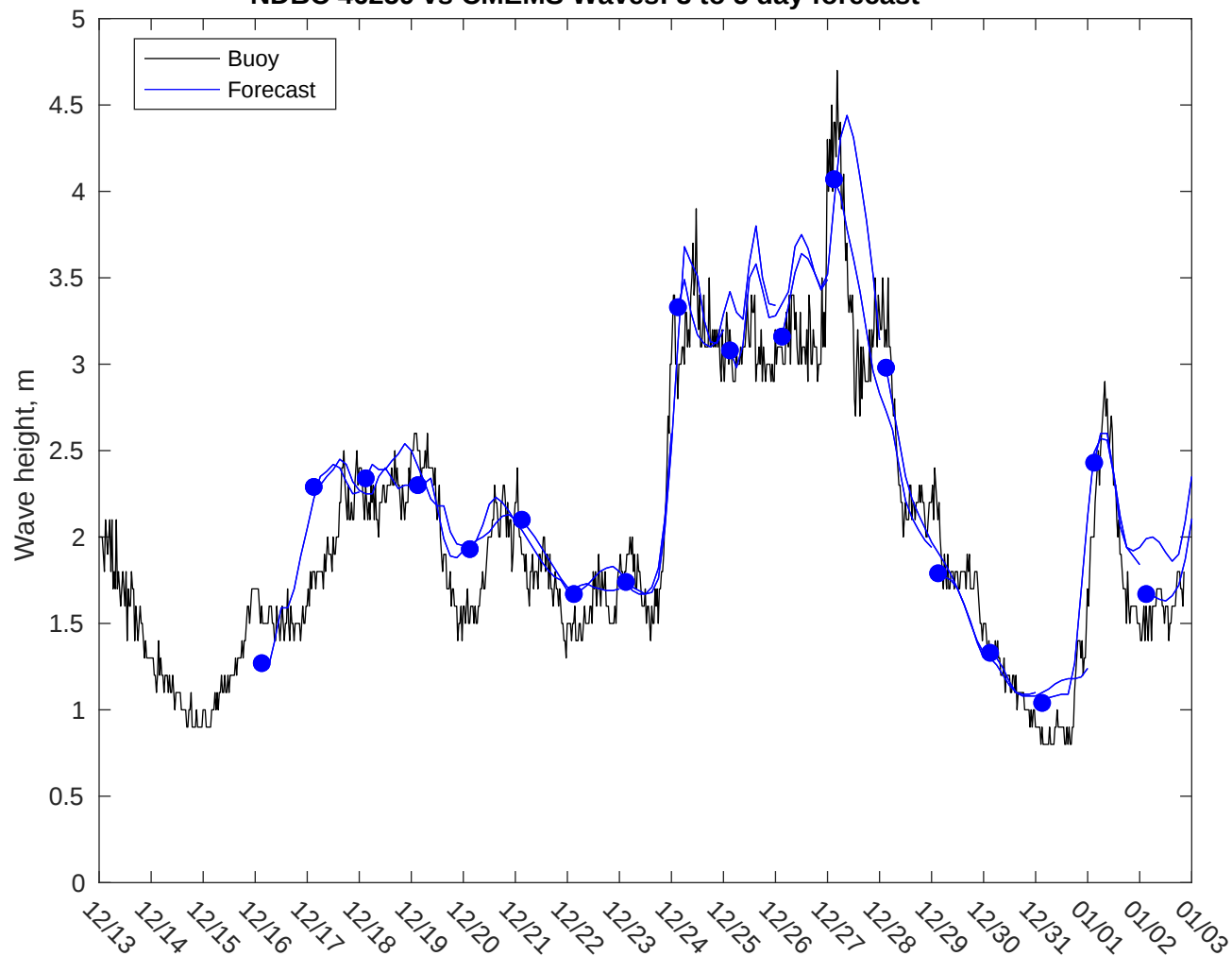
NDBC 46259 vs CMEMS Waves: 3 to 5 day forecast
