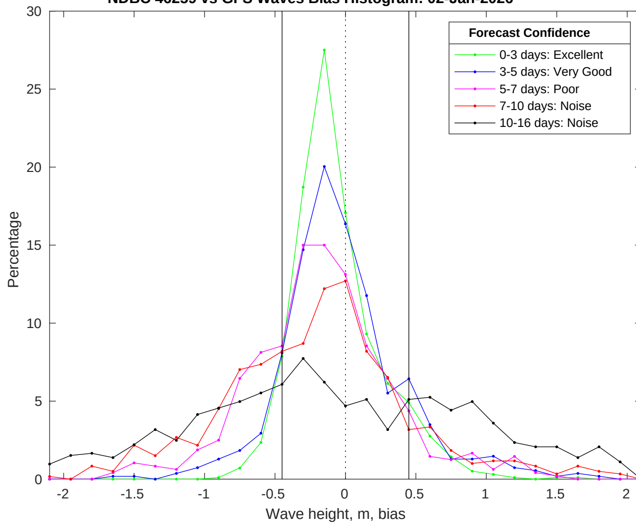
NDBC 46259 vs GFS Waves Bias Histogram: 02-Jan-2026
