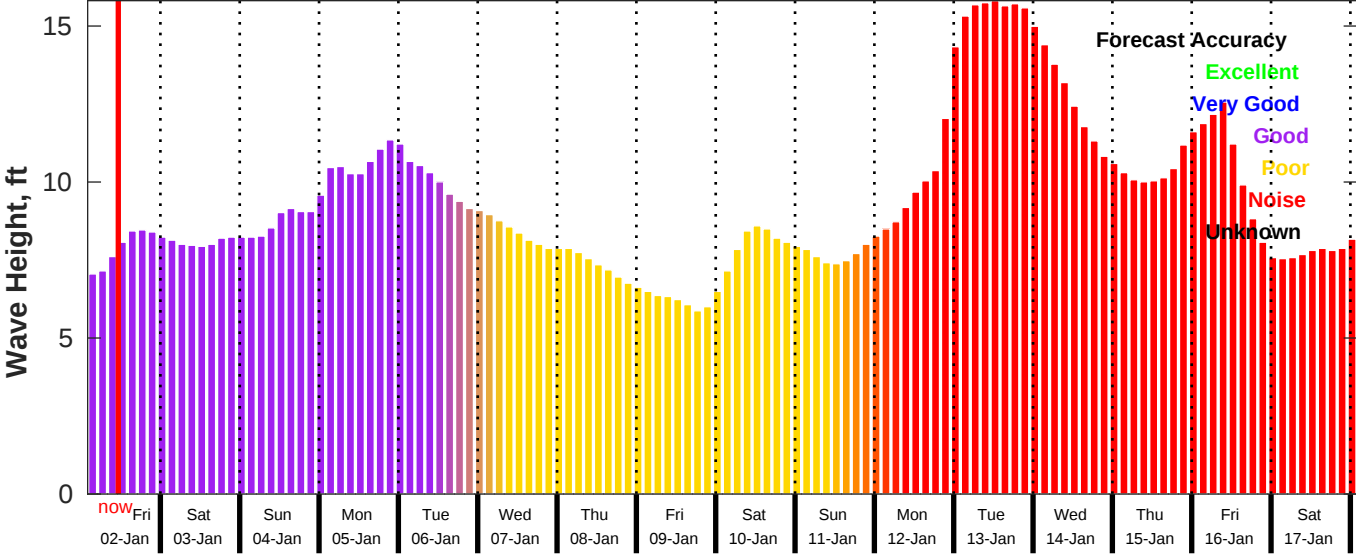
GFS Wave Forecast for NDBC 51000 from 02-Jan-2026 02:00:00 to 18-Jan-2026 02:00:00
