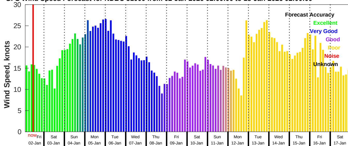
GFS Wind Speed Forecast for NDBC 51000 from 02-Jan-2026 02:00:00 to 18-Jan-2026 02:00:00
