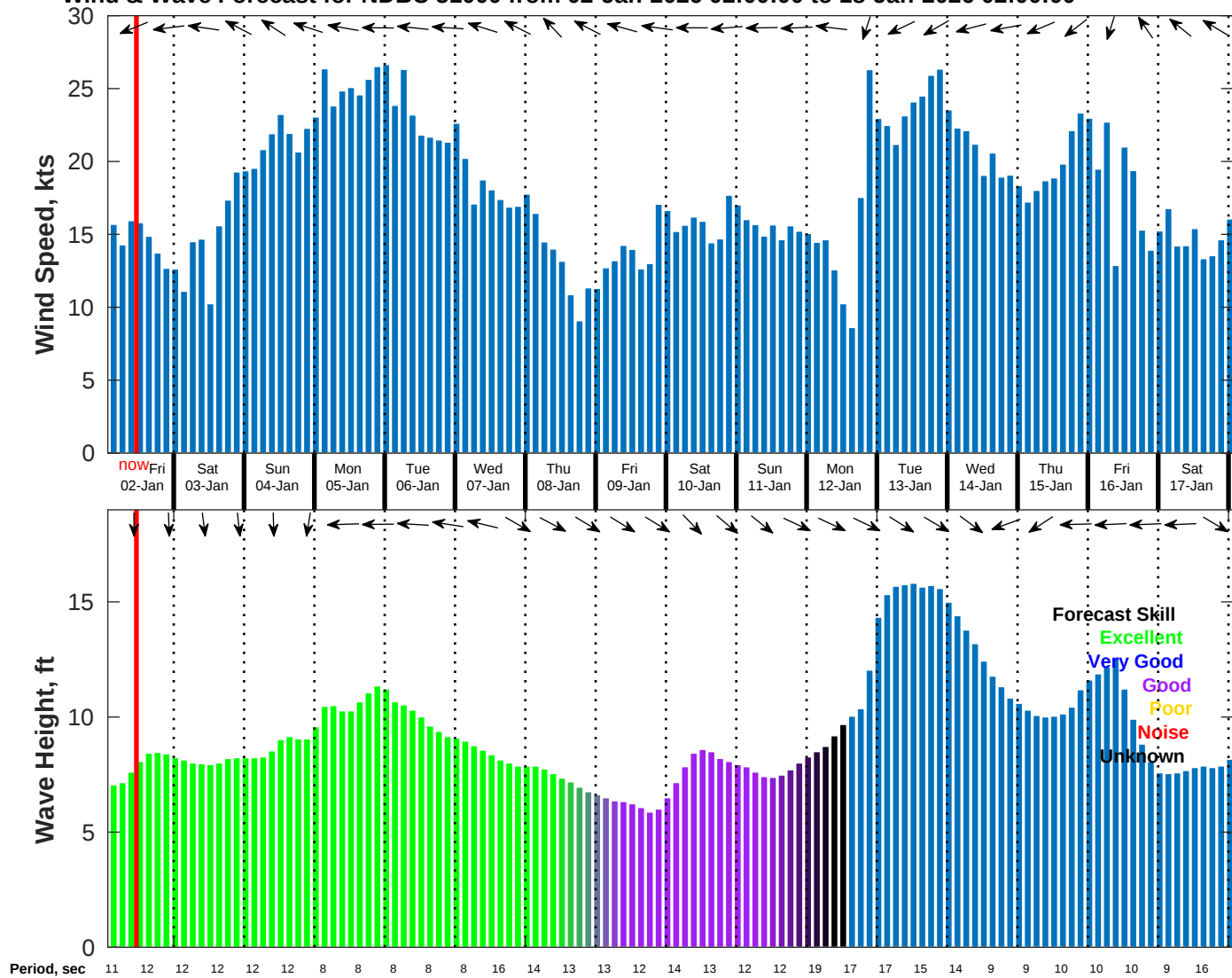
Wind & Wave Forecast for NDBC 51000 from 02-Jan-2026 02:00:00 to 18-Jan-2026 02:00:00
