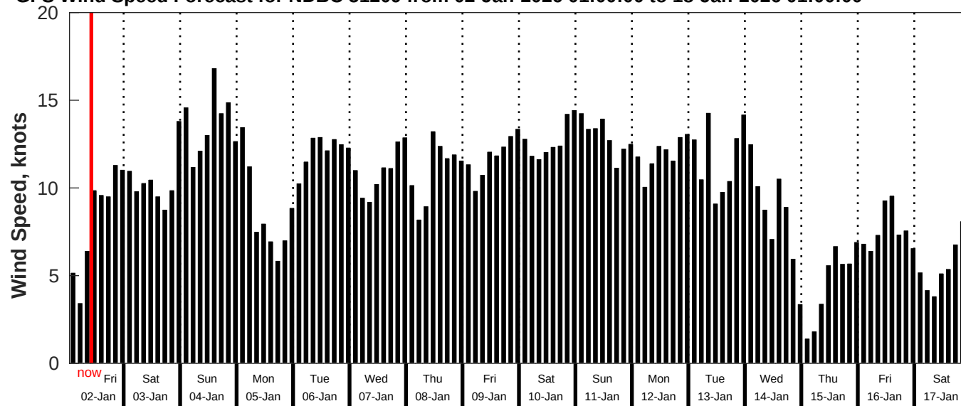
GFS Wind Speed Forecast for NDBC 51209 from 02-Jan-2026 01:00:00 to 18-Jan-2026 01:00:00
