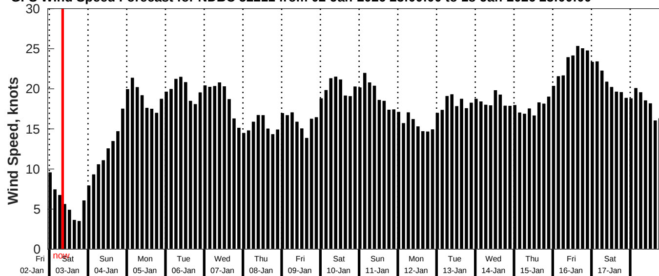
GFS Wind Speed Forecast for NDBC 52211 from 02-Jan-2026 23:00:00 to 18-Jan-2026 23:00:00
