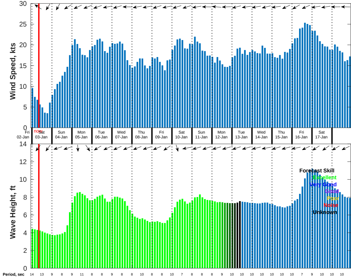
Wind & Wave Forecast for NDBC 52211 from 02-Jan-2026 23:00:00 to 18-Jan-2026 23:00:00
