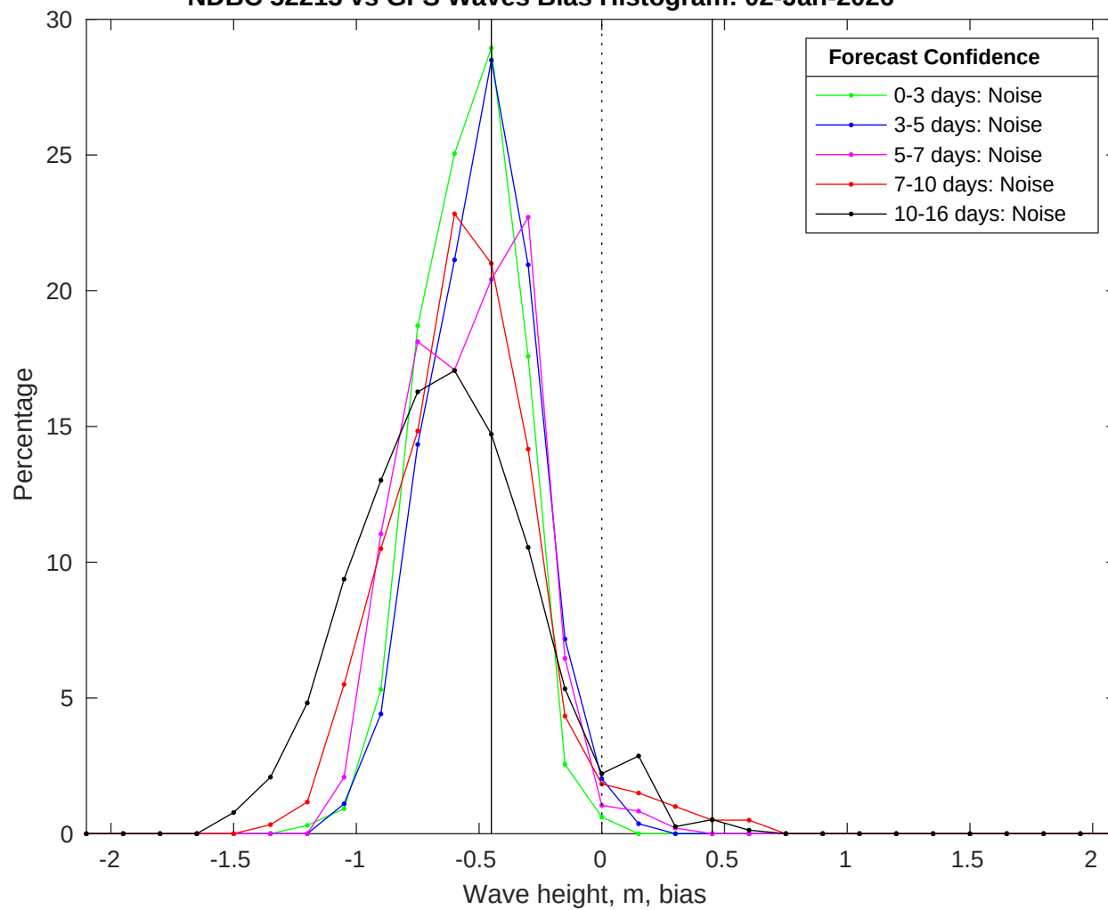
NDBC 52213 vs GFS Waves Bias Histogram: 02-Jan-2026
