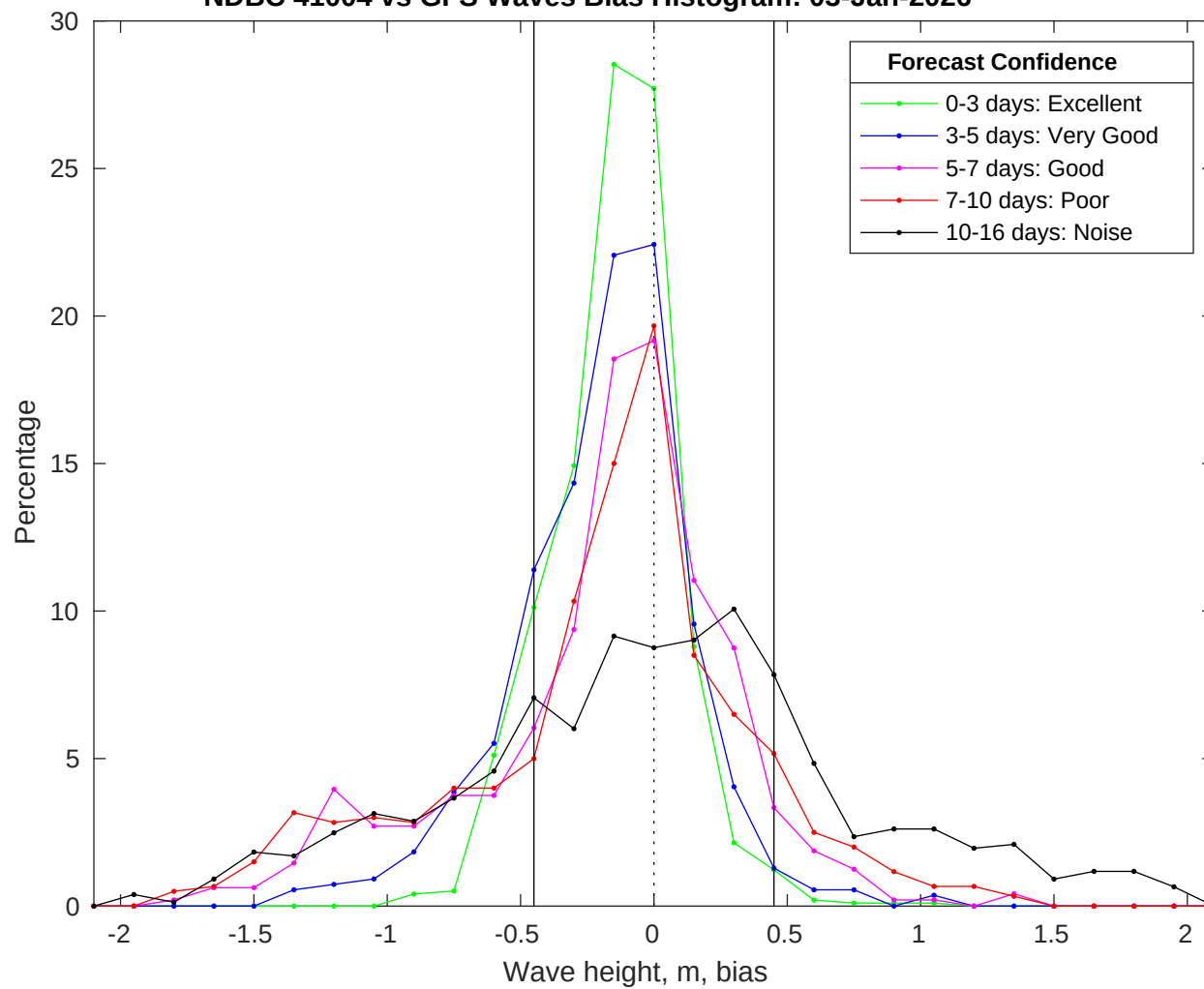
NDBC 41004 vs GFS Waves Bias Histogram: 03-Jan-2026
