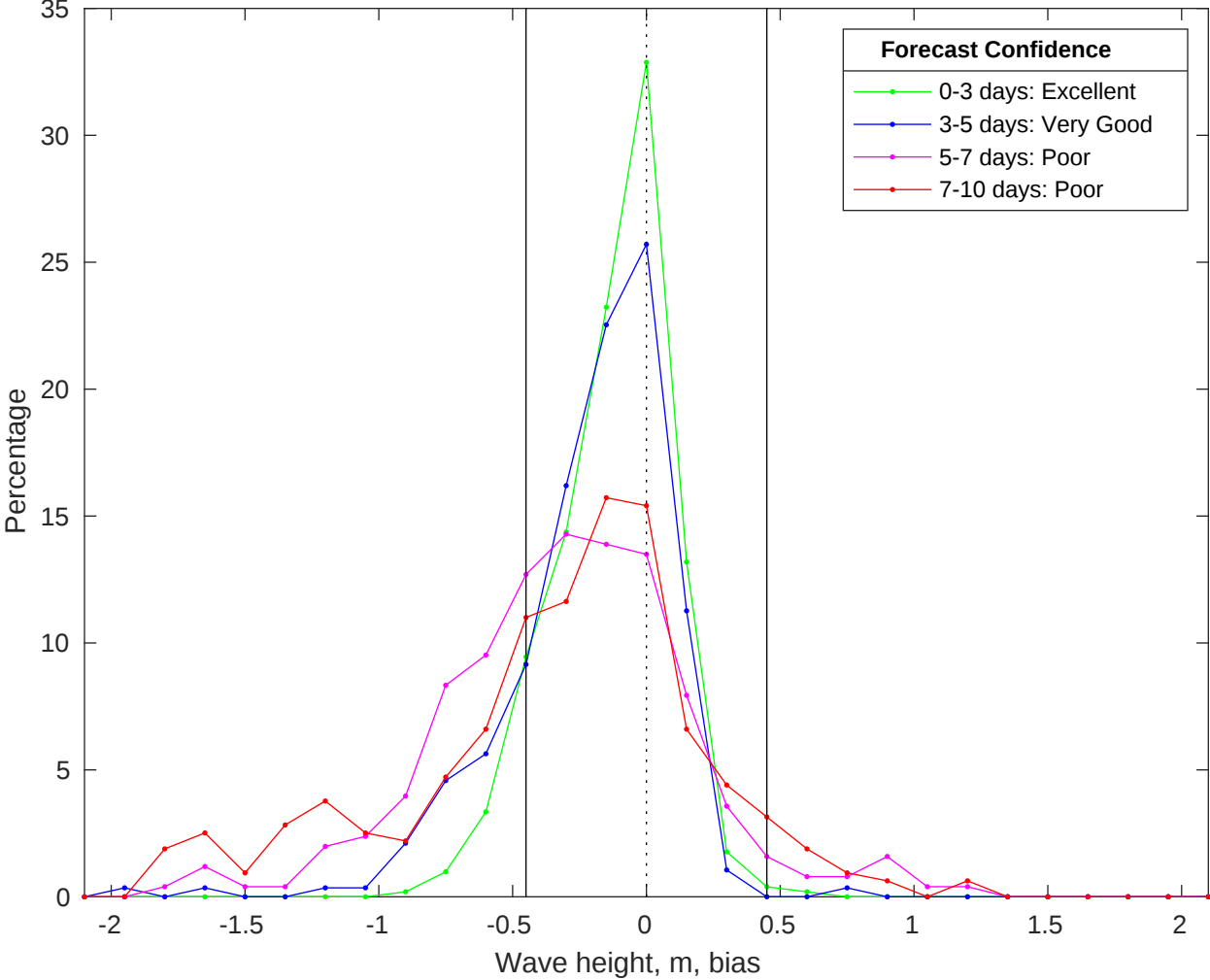
NDBC 41013 vs CMEMS Waves Bias Histogram: 03-Jan-2026
