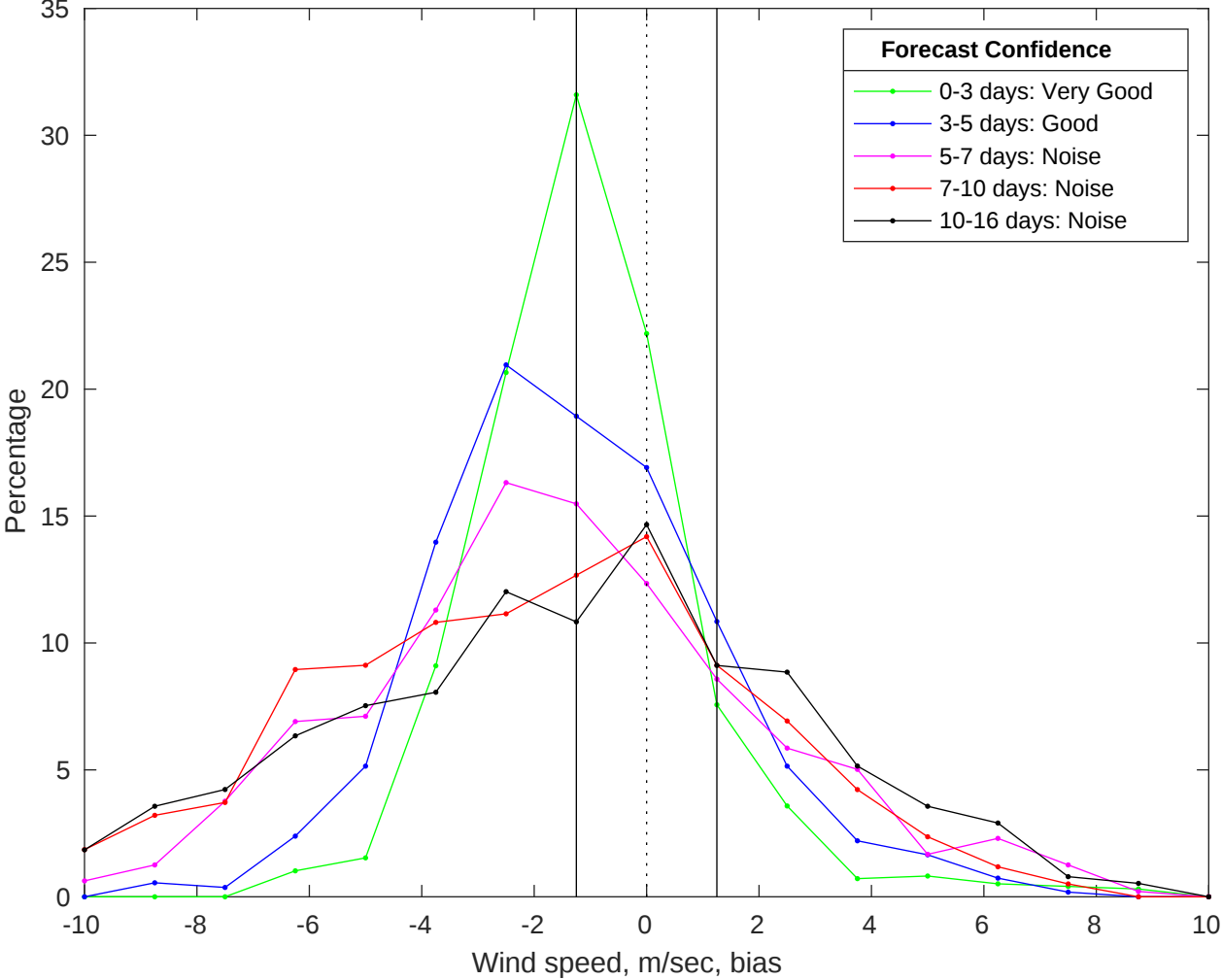
NDBC 41013 vs GFS Winds Bias Histogram: 03-Jan-2026
