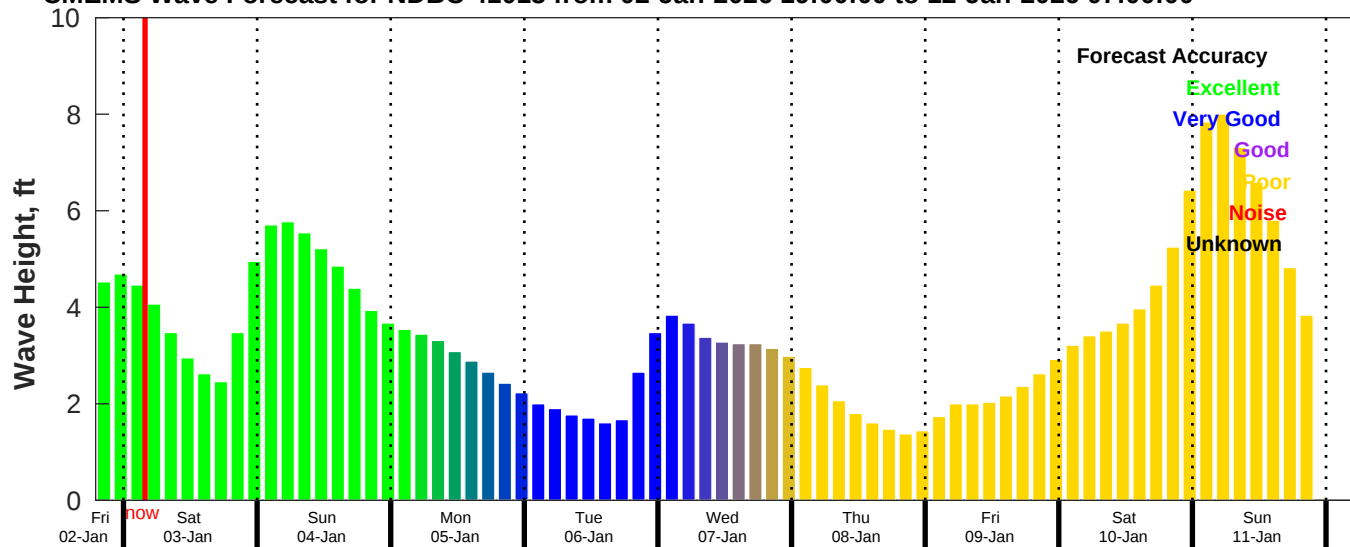
CMEMS Wave Forecast for NDBC 41013 from 02-Jan-2026 19:00:00 to 12-Jan-2026 07:00:00
