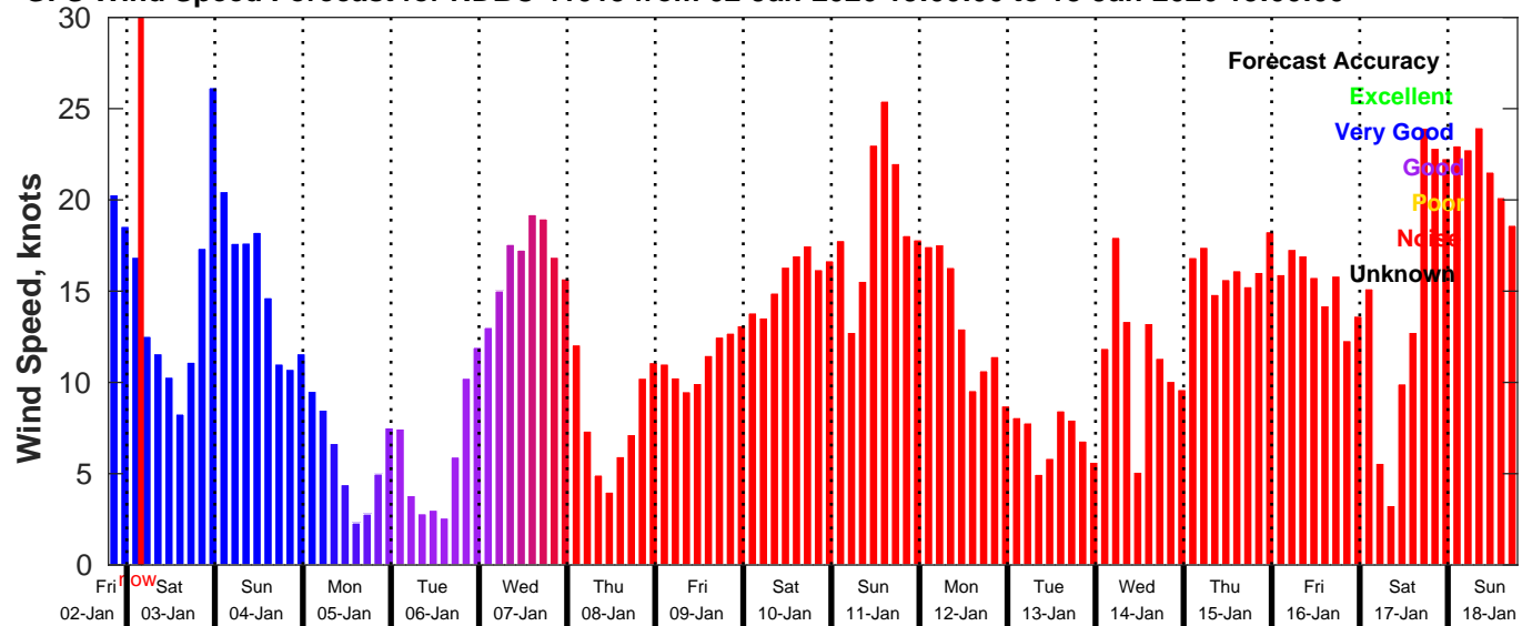
GFS Wind Speed Forecast for NDBC 41013 from 02-Jan-2026 19:00:00 to 18-Jan-2026 19:00:00
