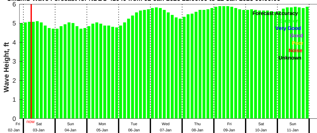
CMEMS Wave Forecast for NDBC 41040 from 02-Jan-2026 21:00:00 to 12-Jan-2026 09:00:00
