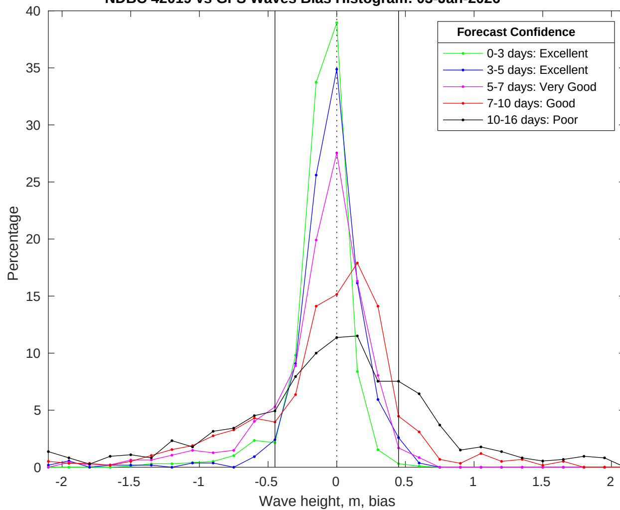
NDBC 42019 vs GFS Waves Bias Histogram: 03-Jan-2026
