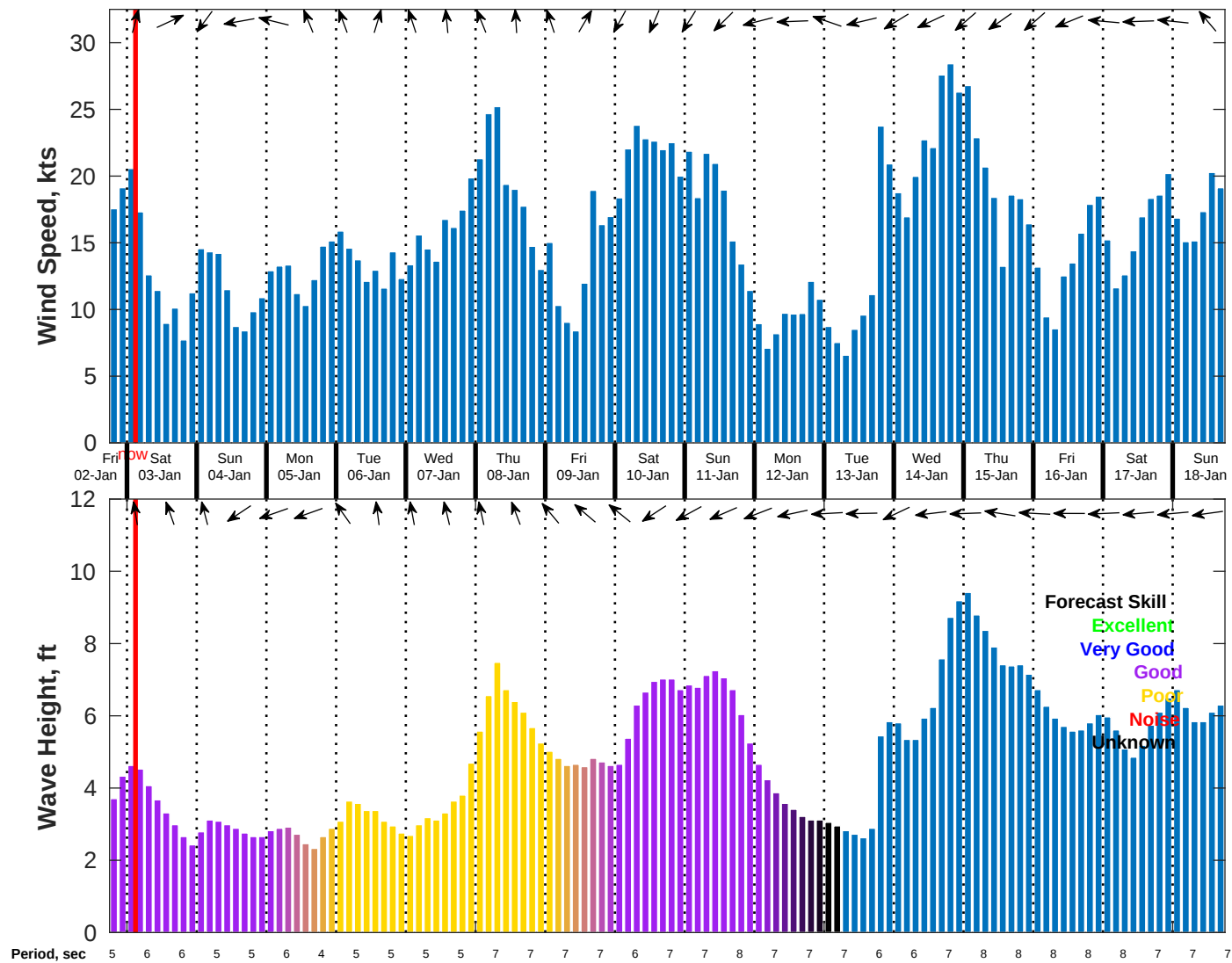
Wind & Wave Forecast for NDBC 42020 from 02-Jan-2026 18:00:00 to 18-Jan-2026 18:00:00
