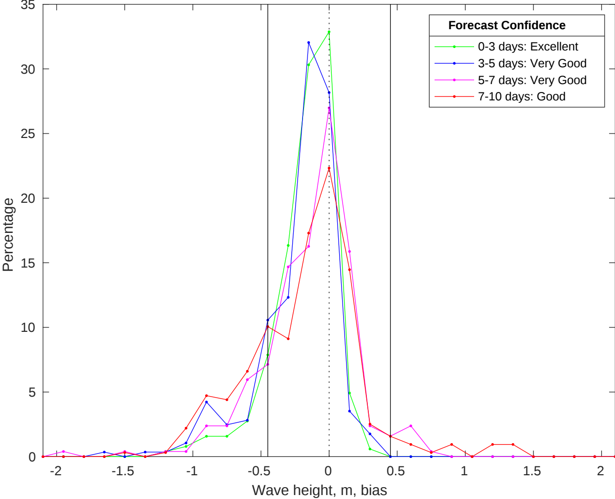
NDBC 42040 vs CMEMS Waves Bias Histogram: 03-Jan-2026
