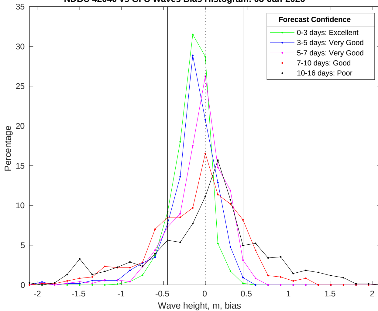
NDBC 42040 vs GFS Waves Bias Histogram: 03-Jan-2026
