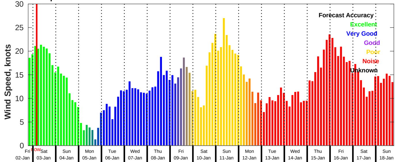
GFS Wind Speed Forecast for NDBC 42040 from 02-Jan-2026 19:00:00 to 18-Jan-2026 19:00:00
