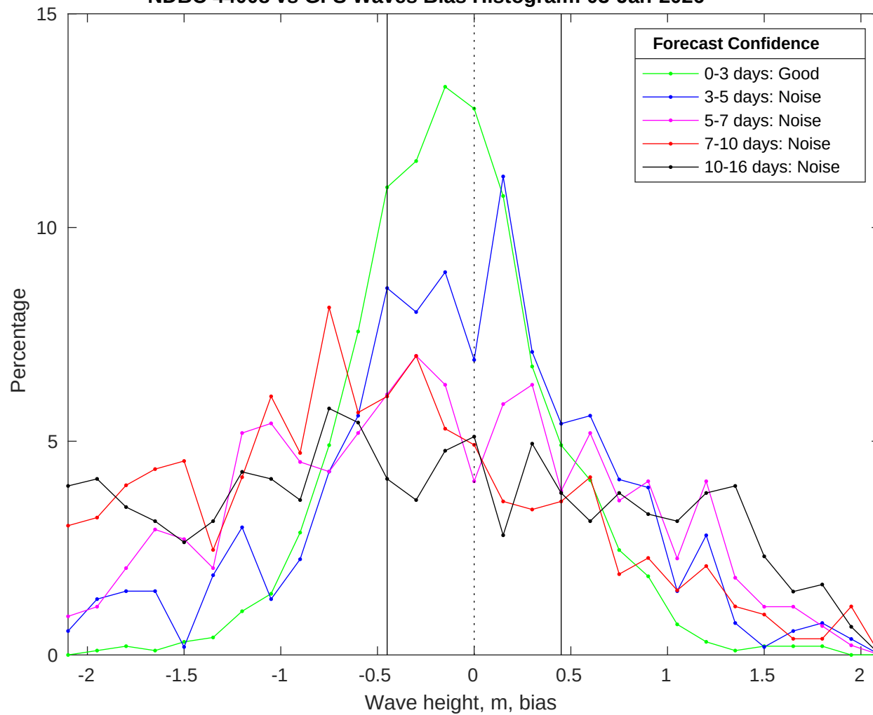
NDBC 44008 vs GFS Waves Bias Histogram: 03-Jan-2026
