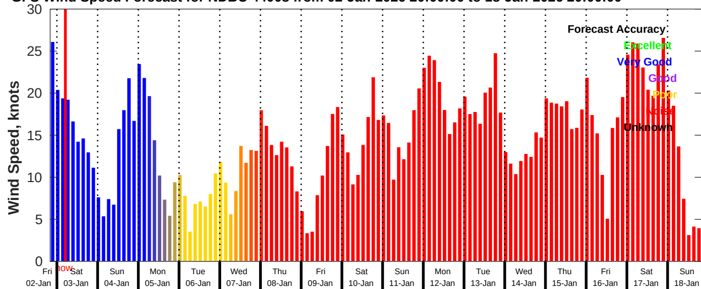
GFS Wind Speed Forecast for NDBC 44008 from 02-Jan-2026 20:00:00 to 18-Jan-2026 20:00:00
