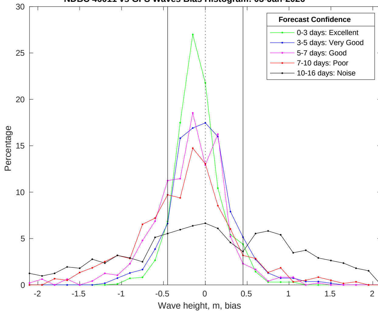
NDBC 46011 vs GFS Waves Bias Histogram: 03-Jan-2026
