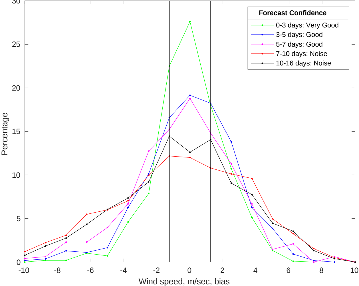
NDBC 46011 vs GFS Winds Bias Histogram: 03-Jan-2026
