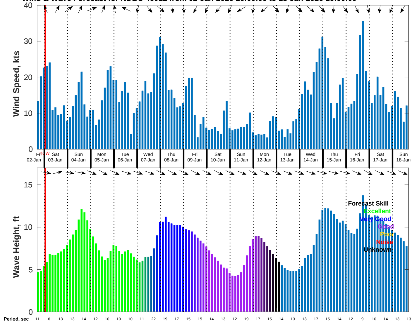
Wind & Wave Forecast for NDBC 46011 from 02-Jan-2026 16:00:00 to 18-Jan-2026 16:00:00
