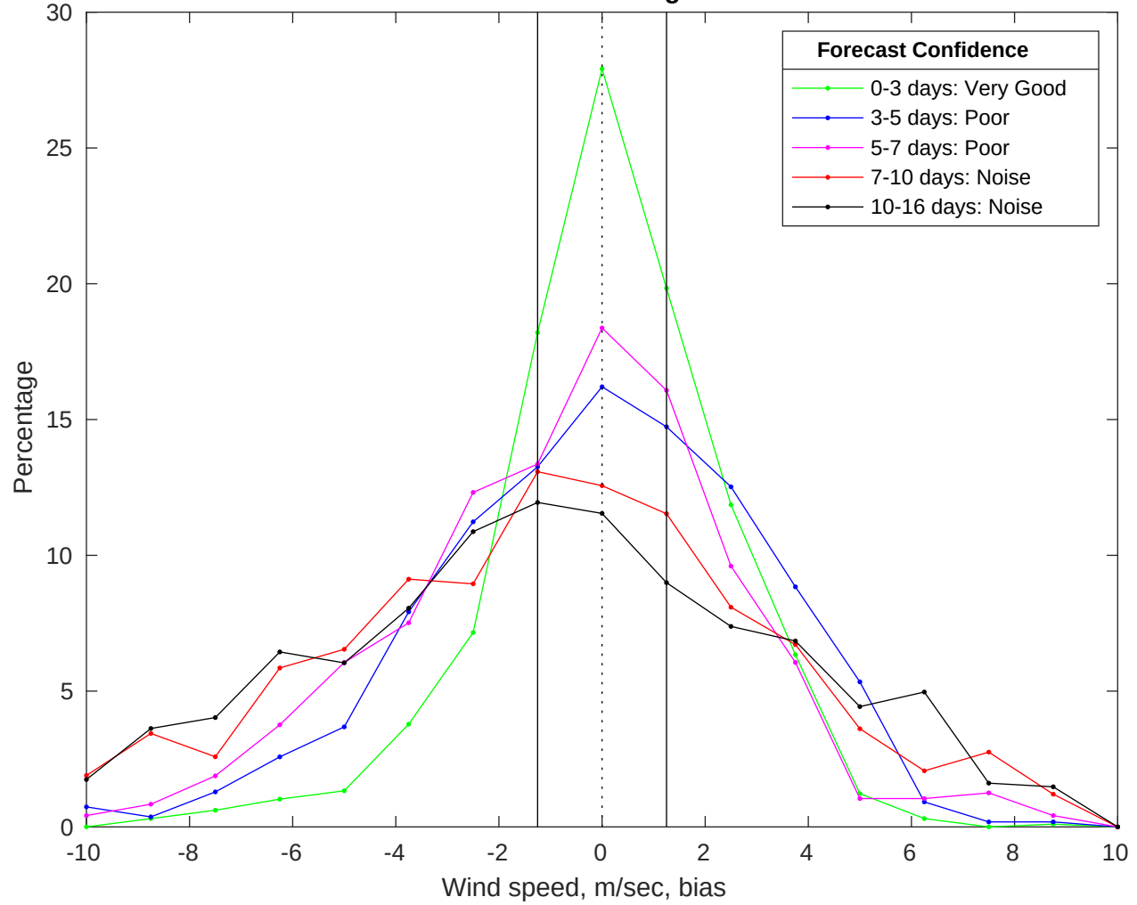
NDBC 46028 vs GFS Winds Bias Histogram: 03-Jan-2026
