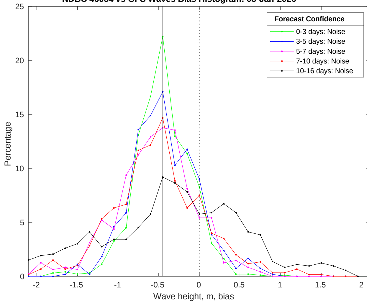
NDBC 46054 vs GFS Waves Bias Histogram: 03-Jan-2026
