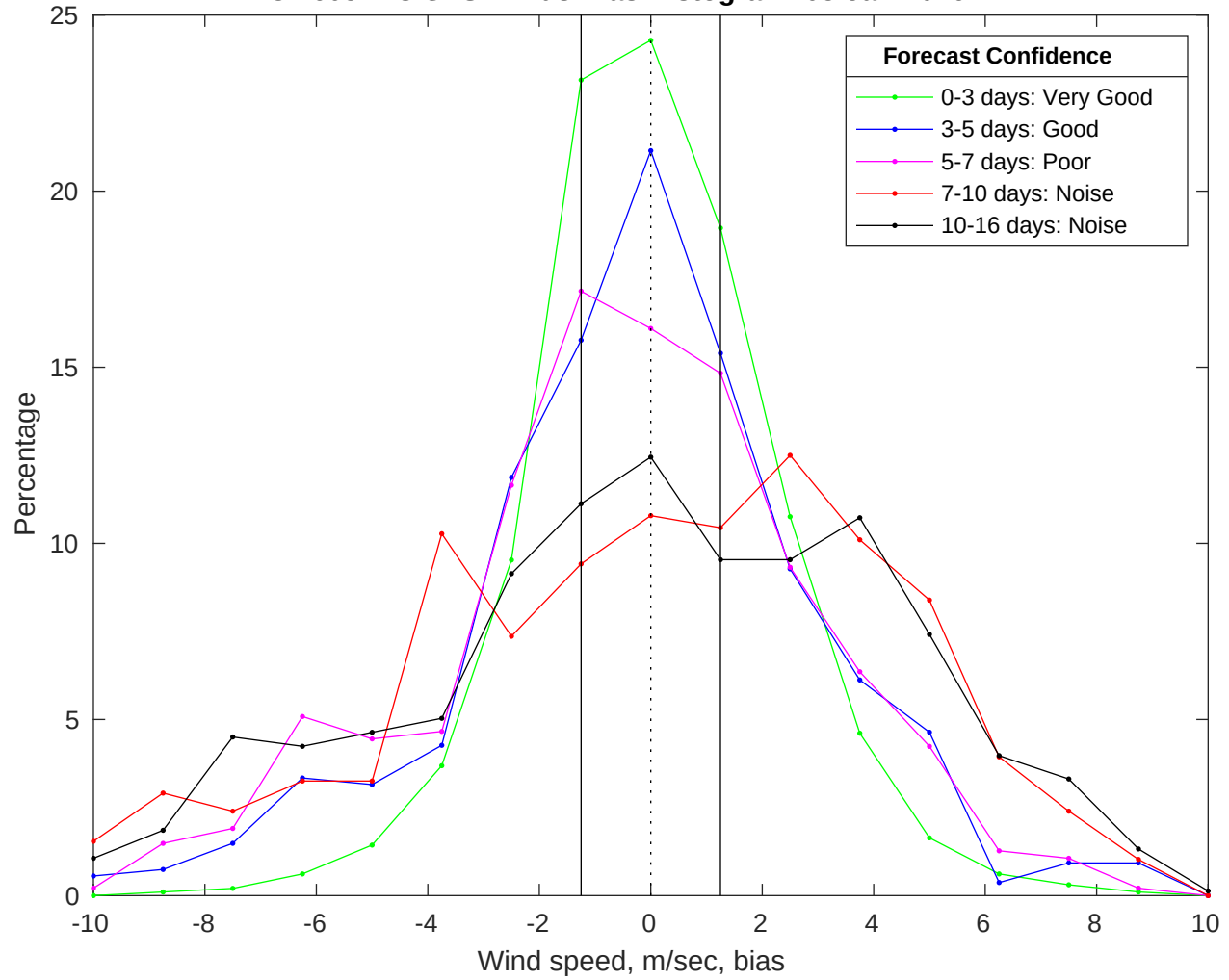
NDBC 46054 vs GFS Winds Bias Histogram: 03-Jan-2026
