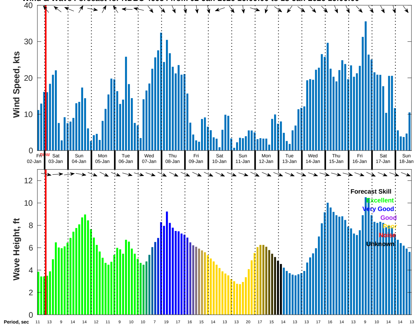
Wind & Wave Forecast for NDBC 46054 from 02-Jan-2026 16:00:00 to 18-Jan-2026 16:00:00
